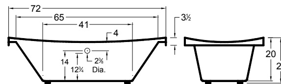
All bathtub dimensions are \pm 1/2'' .
